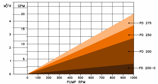
UNIBLOC®-PD SIZE 200-0-275 PUMP CAPACITY CHART
